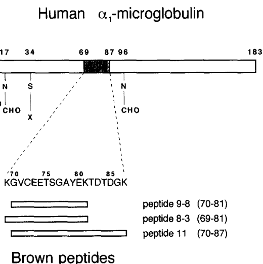
Fig. 1. Schematic representation of human \alpha_1 -m. The 183-amino acid polypeptide is substituted with one O-linked carbohydrate moiety (CHO) bound to the threonine residue at position 5 and two N-linked carbohydrate moieties bound to the asparagine residues at positions 17 and 96. The cysteine residue at position 34 is linked to an unknown substance (X). The three yellow-brown peptides 9–8, 8–3 and 11 were isolated as described in section 2.
