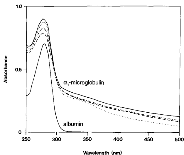
Fig. 3. Absorbance spectrum of \alpha_1 -m from various sources. The light absorbance was measured at a protein concentration of approximately 0.5 mg/ml in PBS. The human \alpha_1 -m homologue was isolated from urine (···) or HepG2 cell culture medium (—), and the rat \alpha_1 -m homologue from urine (---) or baculovirus-transfected insect cells (-·-·-). The lower unbroken line shows the spectrum of albumin isolated from rat urine.
